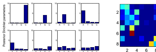
Figure 4. (a) Dirichlet hyperparameters (of components 1-8 from left to right, top to bottom). (b) Markov transition matrix.
