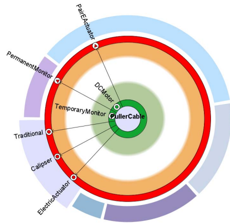
Fig. 12: FROG of PullerCable feature with a filter hiding Independent zone features to illustrate great impact on other features
