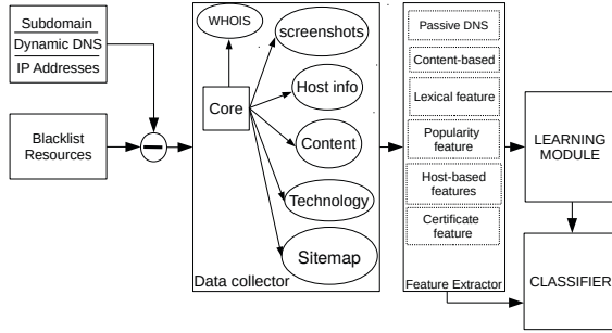
Figure 1: COMAR system structure.
