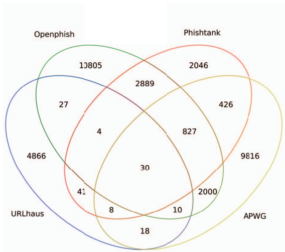
Figure 8: Venn diagram of the collected URLs from four blacklists.
