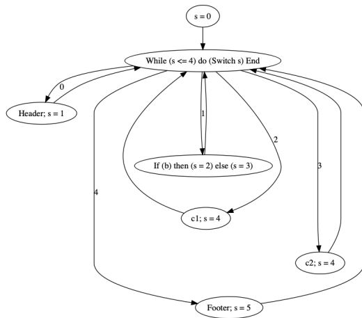
Figure 2. Flattened If-Then-Else
