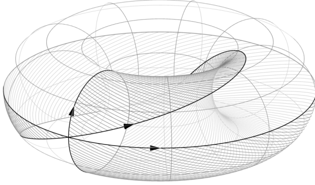
Fig. 2. A homotopy.
