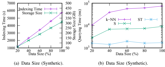
Fig. 14. Scalability of JUST.
