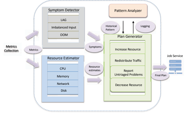
Fig. 4: The architecture of Turbine's Auto Scaler.
