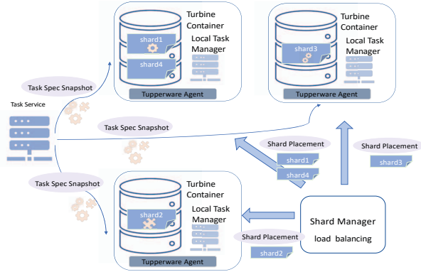
Fig. 3: Turbine's Task Management with a two-level distributed task scheduling and load balancing.
