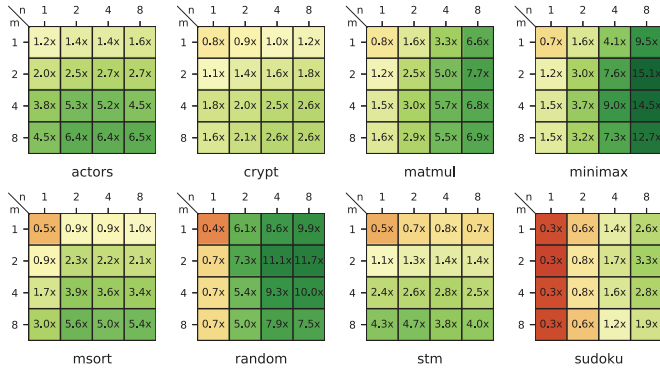
Fig. 5. Speedups for the MODCONC benchmarks, relative to the sequential implementation. Horizontally (left-to-right), we increase the number of workers for MODCONC inter-component analysis. Vertically (top-to-bottom), we increase the number of workers per intra-component (MODF) analysis.
