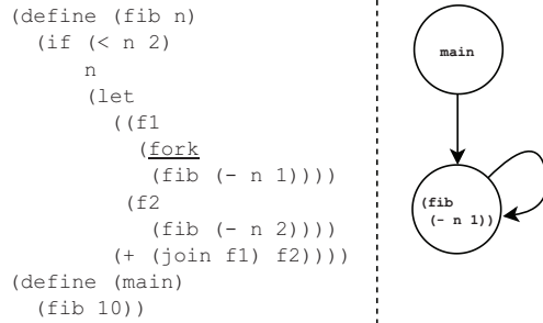
Fig. 2. A MODCONC analysis example (left: the Scheme program under analysis; right: a graph computed by a context-insensitive MODCONC analysis, showing how threads fork other threads in the program).
