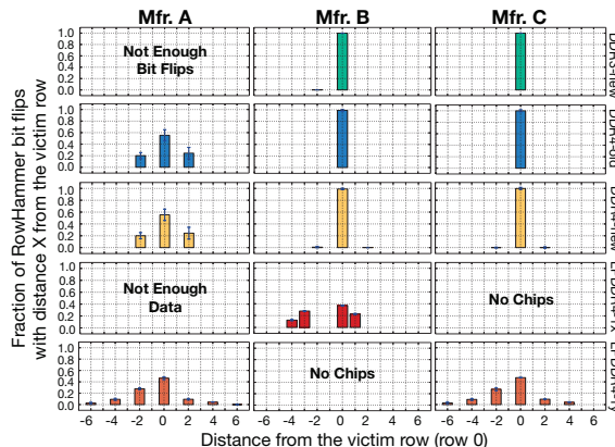
Figure 6: Distribution of RowHammer bit flips across row offsets from the victim row.
