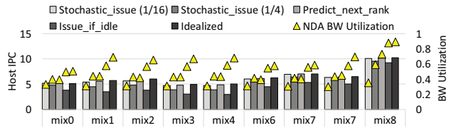
Fig. 12: Stochastic issue and next-rank prediction impact.
