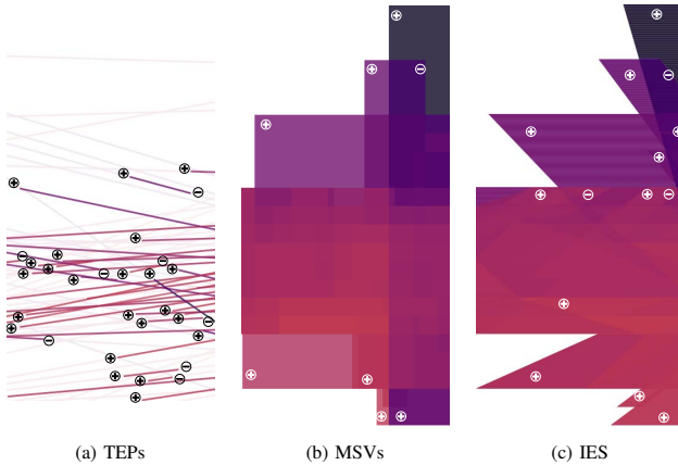
Fig. 9. A cut-off of graph G4 between timepoint time_36 and timepoint time_70 visualized using TEPs, MSVs, and IES. More link events are identified in TEPs.
