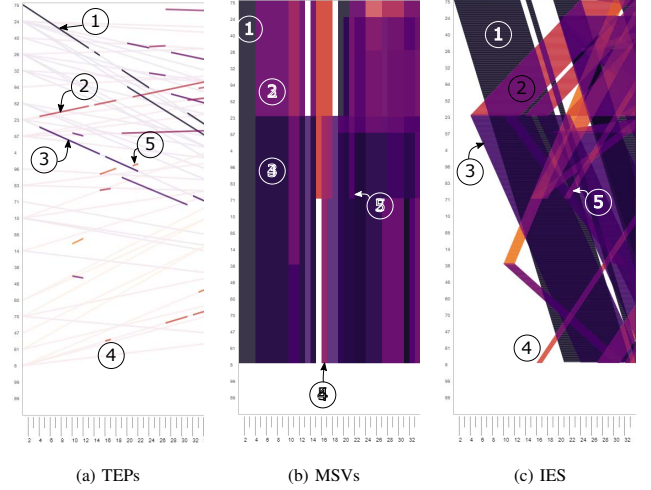
Fig. 10. A cut-off of the first 33 timepoints from graph G5 visualized using TEPs, MSVs, and IES. Links ①, ②, ③, and ④ exhibit a periodic behavior.
