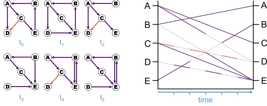
Fig. 1. Comparison between small multiples of node-link diagrams (left) and time-aligned edge plots (right). Edges over time are depicted by a single line in time-aligned edge plots.
