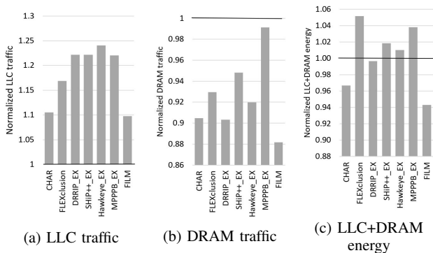
Fig. 8: The traffic and energy of shared memory resource (LLC and DRAM) of FILM and other schemes. Results normalized to TC-UC. The lower the better.
