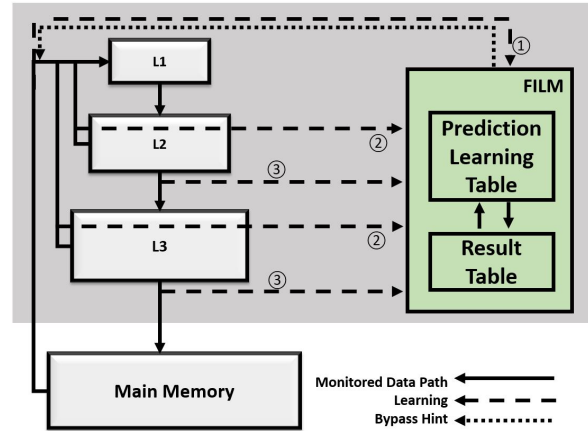
Fig. 3: Overview of the proposed FILM system
