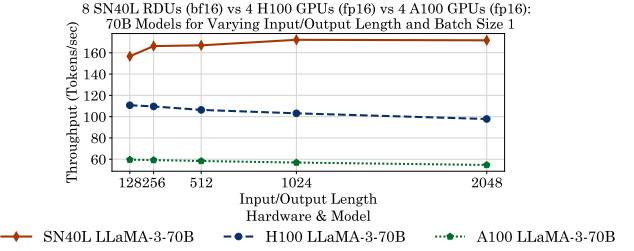
Fig. 19: Throughput Comparison of 70B Model on 8 SN40L RDUs with 4 A100 and 4 H100 GPUs
