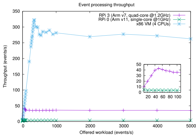
Fig. 5. Event processing throughput for different candidate edge host technologies under increasing workload.
