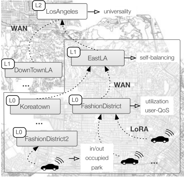
Fig. 4. Monitoring scenario over Los Angeles; events are emitted through LoRa from IoT devices to local edge nodes (in grey). Those in turn propagate property evaluations to a city-wide node (top). The box denotes the architecture-critical levels L0 and L1 considered for evaluation.
