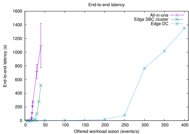
Fig. 6. Mean end-to-end latency (over 95% confidence intervals) as a function of event workload for different deployment scenarios.
