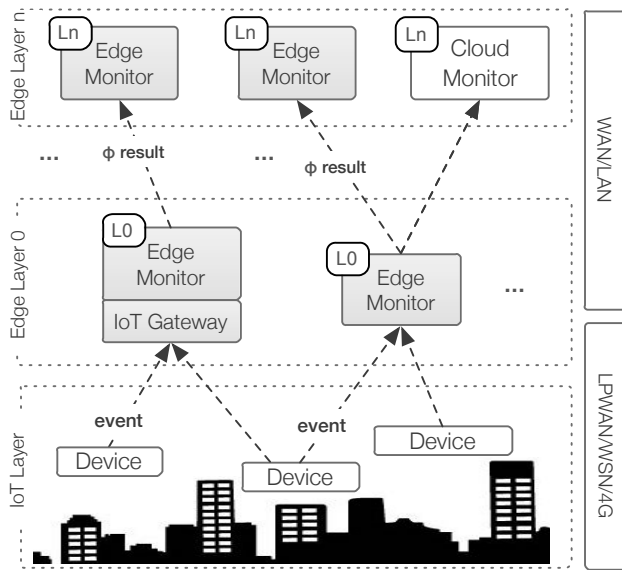
Fig. 1. Edge-based Monitoring Architecture. IoT devices in the range of local edge monitors emit events. Edge monitors are responsible for runtime verification and are deployed in a hierarchical structure, where verdicts of property evaluations are propagated.
