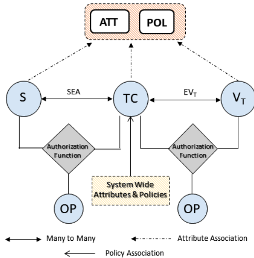
Figure 3: A Conceptual AB-ITS Communication Model
