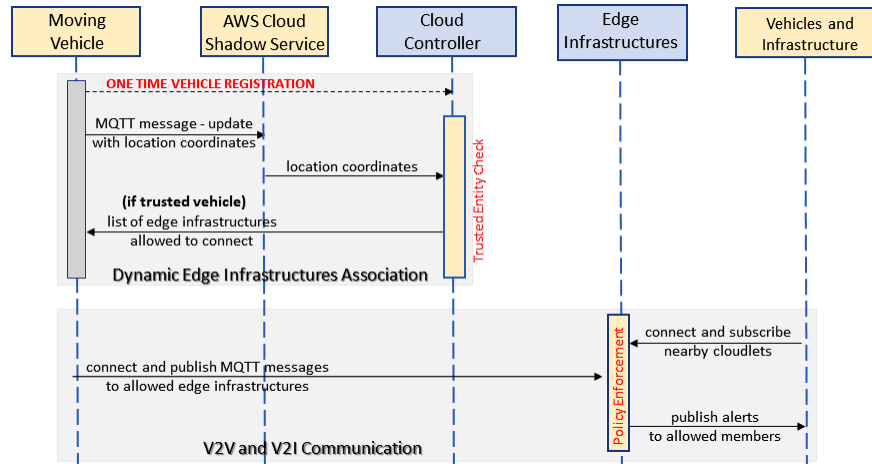
Figure 7: Sequence Diagram for Cloudlets Supported V2V and V2I Communication
