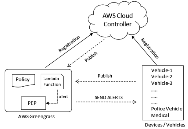
Figure 4: System Architecture
