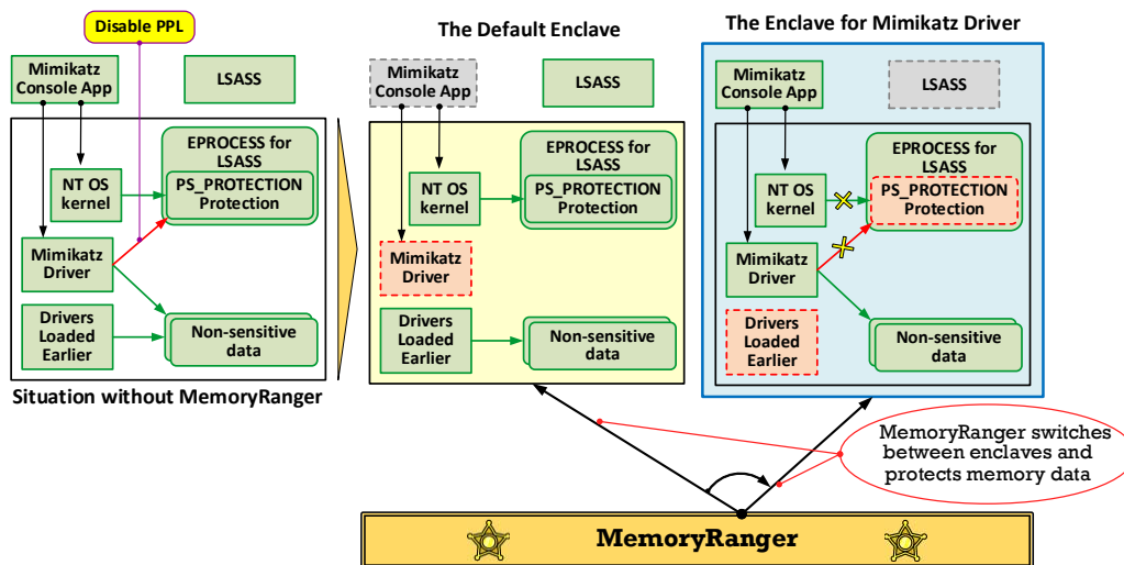
Figure 9. Case 2: MemoryRanger protects the EPROCESS structure of the LSASS process from being patched by Mimikatz driver using two enclaves: the default one for drivers loaded earlier and a separate enclave for newly loaded Mimikatz driver
