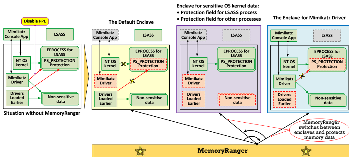
Figure 8. Case 1: MemoryRanger protects the EPROCESS structure of the LSASS process from being patched by Mimikatz driver using three enclaves: the default one for drivers loaded earlier, the enclave for sensitive OS kernel data, and a separate enclave for newly loaded Mimikatz driver
