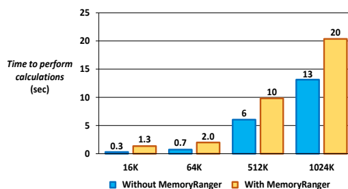
Figure 7. MemoryRanger benchmark assessment: with enabled MemoryRanger the CPU performance degradation is about 50%
