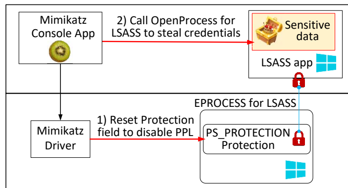
Figure 5. Mimikatz disables PPL protection for the LSASS process in order to acquire the password hashes stored in LSASS process memory
