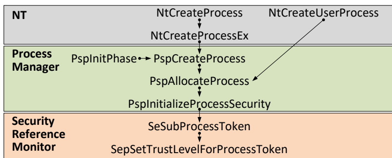
Figure 2. The internals of CreateProcess.
